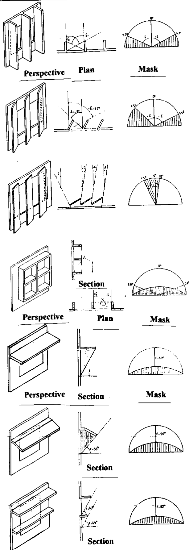
Figure 28. Some examples of the shading devices and shadow masks.
